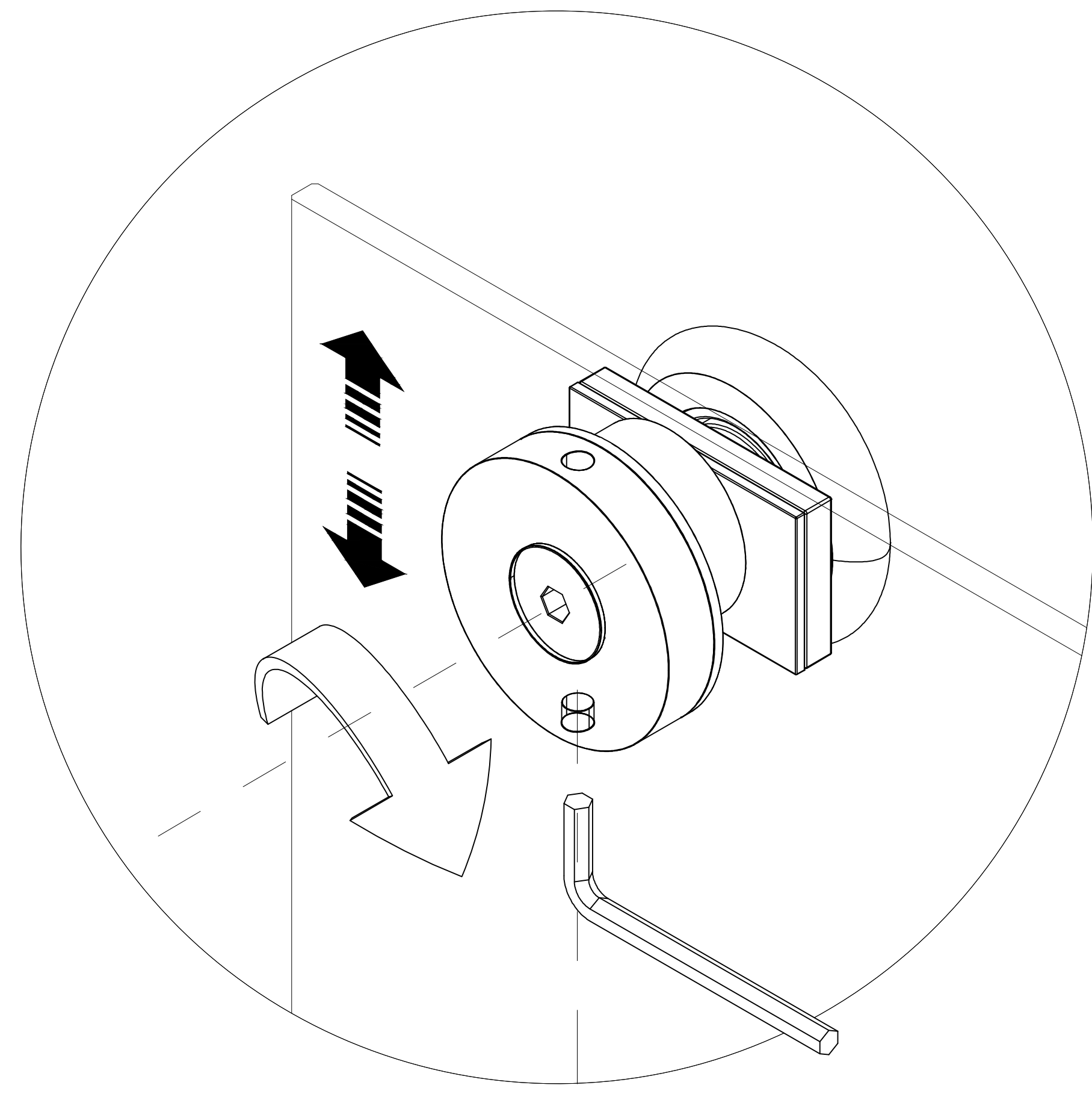
STEP-9-1
